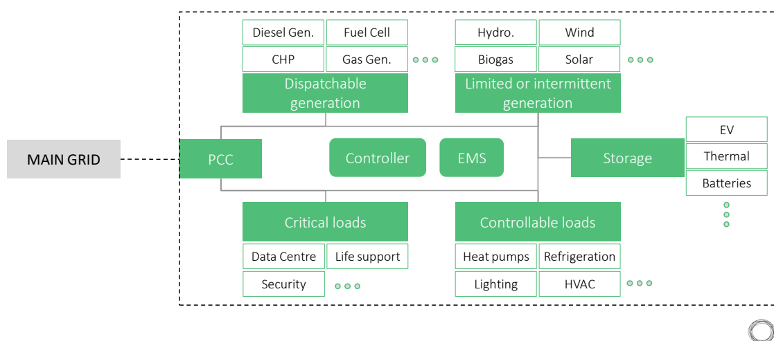
Figure 2 - General representation of a grid-connected microgrid 11
